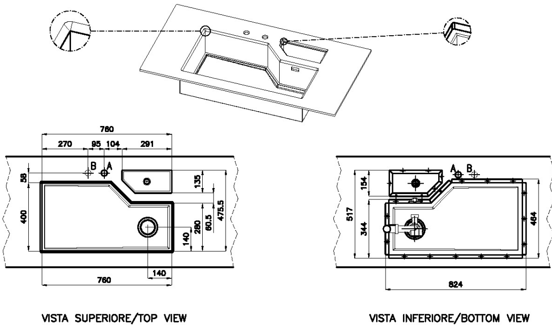
VISTA SUPERIORE/TOP VIEW
